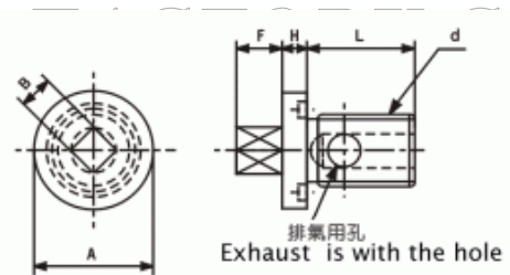
■排氣用螺栓 Bolt for exhausting (CNS 3270-403)
